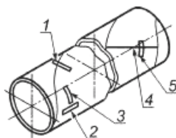
b — Трубы CW, LFW, HFW, LW, SAWL и COWL
